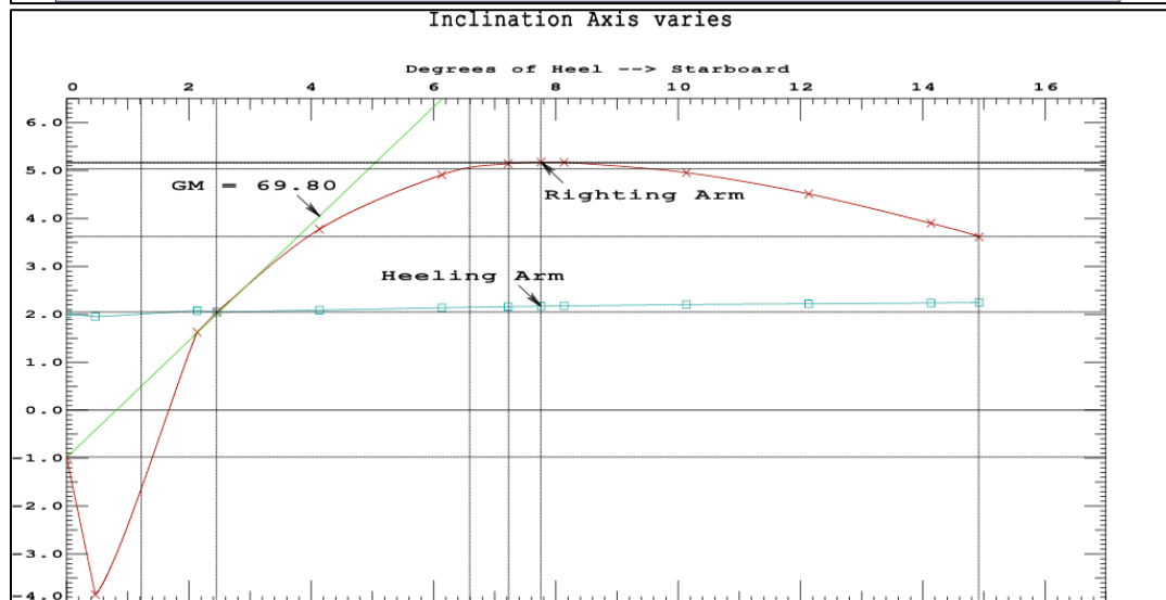
Figure 30: GHS output for varied axis analysis of departure condition with 70-knot winds
