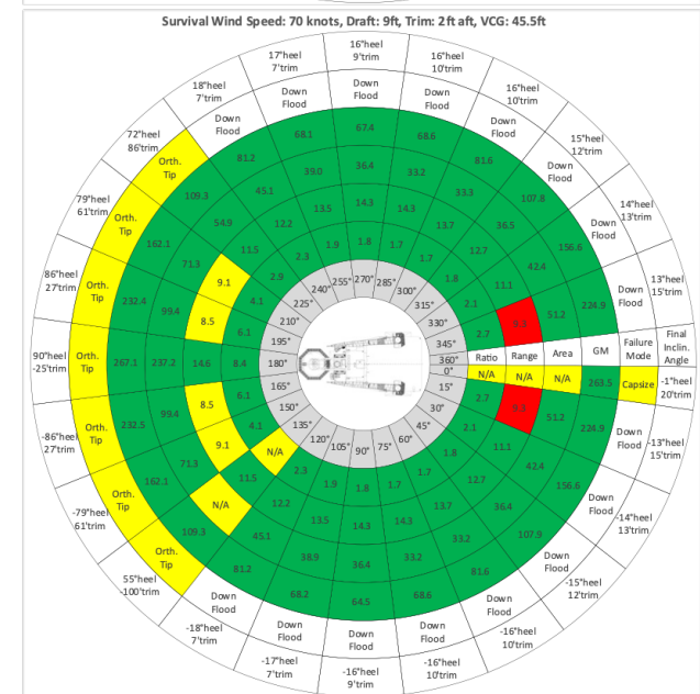
Figure 21: MSC Fixed Interval Analysis Results for 60-knot wind (left) and 70-knot wind (right). 8.5-foot draft (top), 9-foot draft (bottom). Trim is 2 feet
