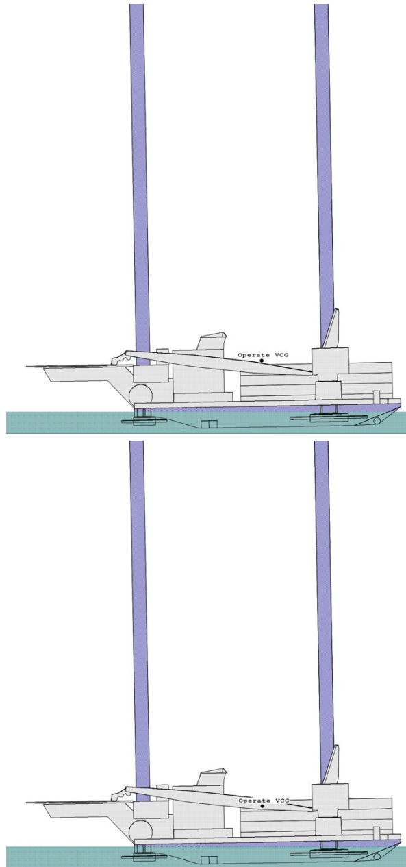
Figure 22: MSC Fixed Interval Analysis Results for 60-knot wind (left) and 70-knot wind (right). 9.5-foot draft (top), 10-foot draft (bottom). Trim is 2 feet
