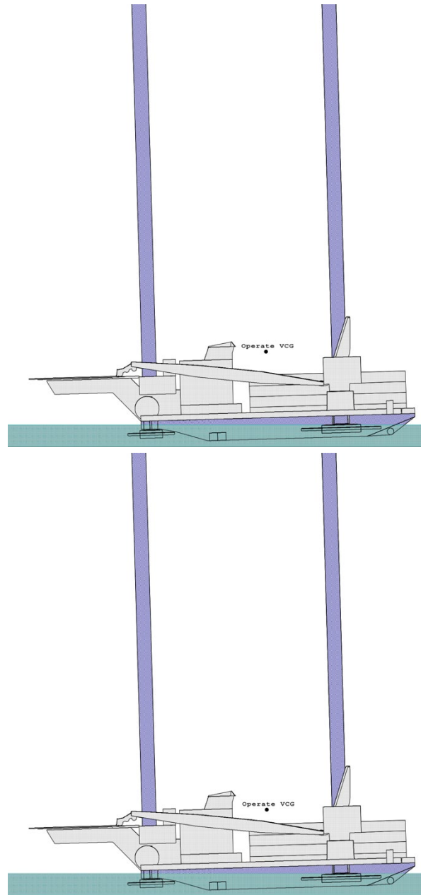
Figure 23: MSC Fixed Interval Analysis Results for 60-knot wind (left) and 70-knot wind (right). 8.5-foot draft (top), 9-foot draft (bottom). Trim is 3 feet
