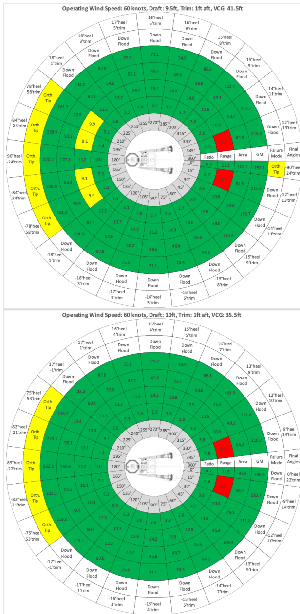
Figure 20: MSC Fixed Interval Analysis Results for 60-knot wind (left) and 70-knot wind (right). 9.5-foot draft (top), 10-foot draft (bottom). Trim is 1-foot
