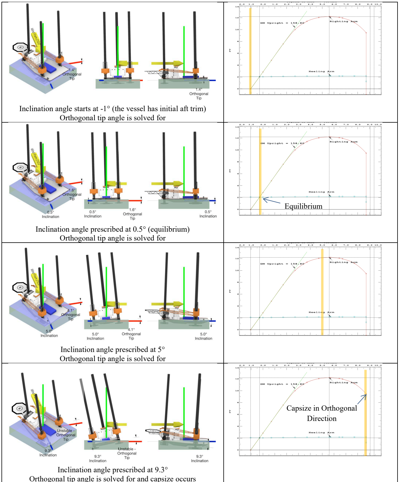
Figure 13: Fixed Axis Method with Winds from 210^\circ Relative for the Casualty Condition with 70 Knot Winds, Demonstrating Fading Stability (failure due to Orthogonal Tipping, Page 630 of Appendix D)
