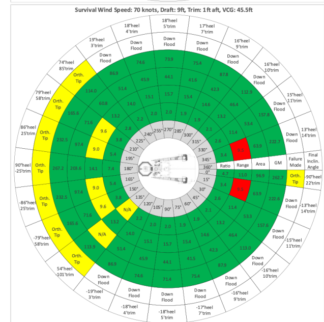
Figure 19: MSC Fixed Interval Analysis Results for 60-knot wind (left) and 70-knot wind (right). 8.5-foot draft (top), 9-foot draft (bottom). Trim is 1-foot
