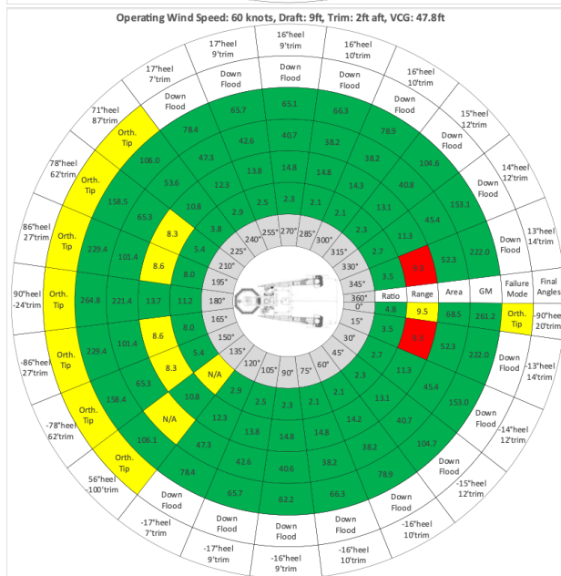
Figure 21: MSC Fixed Interval Analysis Results for 60-knot wind (left) and 70-knot wind (right). 8.5-foot draft (top), 9-foot draft (bottom). Trim is 2 feet
