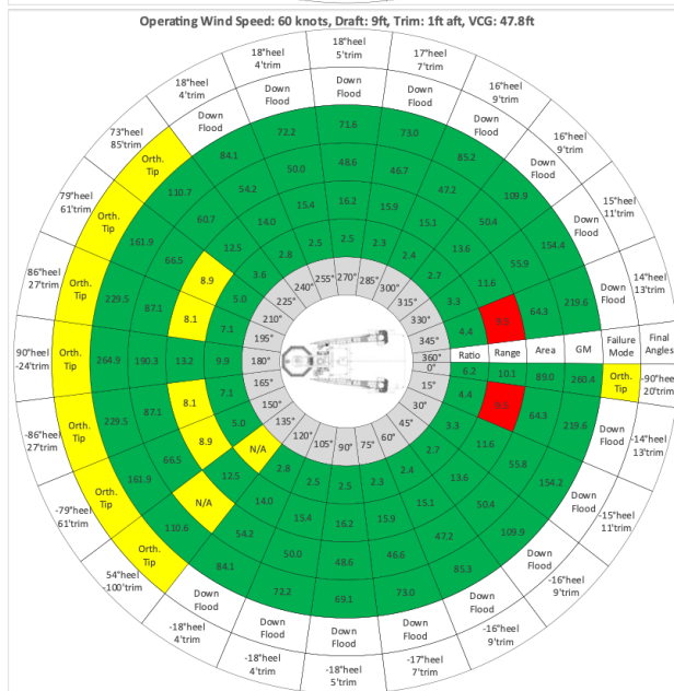
Figure 19: MSC Fixed Interval Analysis Results for 60-knot wind (left) and 70-knot wind (right). 8.5-foot draft (top), 9-foot draft (bottom). Trim is 1-foot
