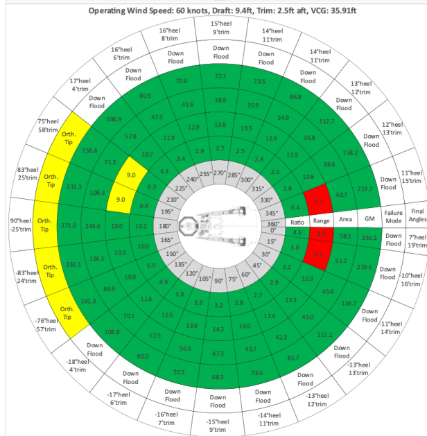
Figure 35: MSC Fixed Interval Analysis Results for 60-knot wind (left) and 70-knot wind (right). Departure Condition (top), Casualty Condition (bottom).
