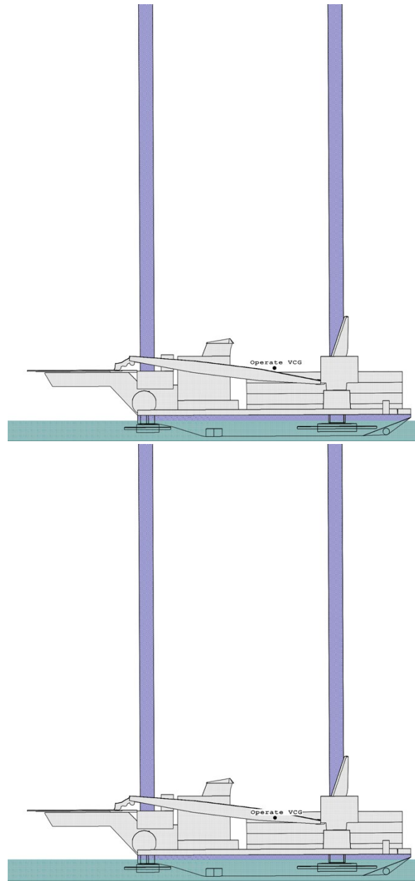
Figure 18: MSC Fixed Interval Analysis Results for 60-knot wind (left) and 70-knot wind (right). 9.5-foot draft (top), 10-foot draft (bottom). Trim is 0.5 feet
