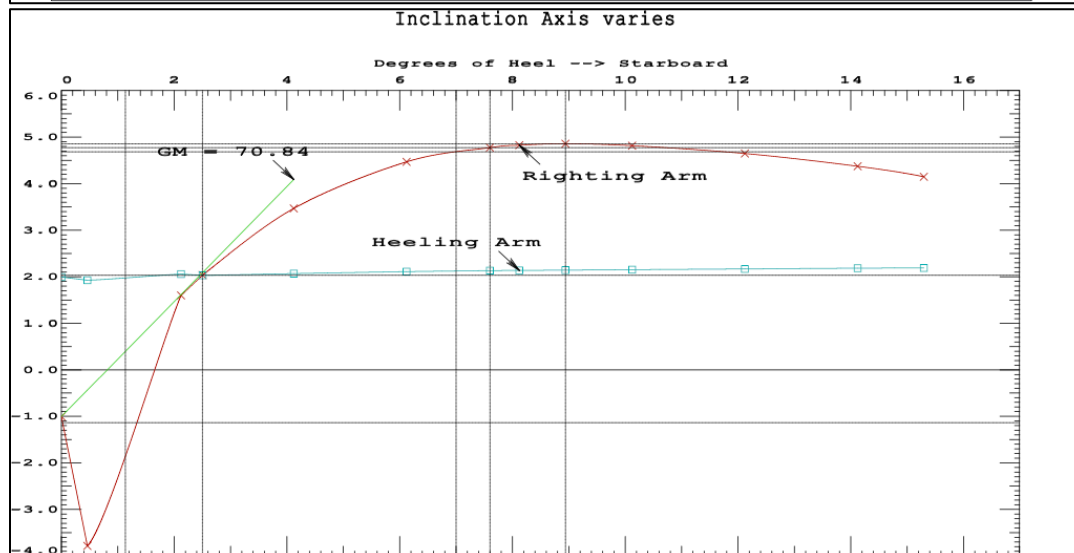
Figure 34: GHS output for varied axis analysis of casualty condition with 70-knot winds. Note that axis angles in GHS are measured clockwise from 270° relative
