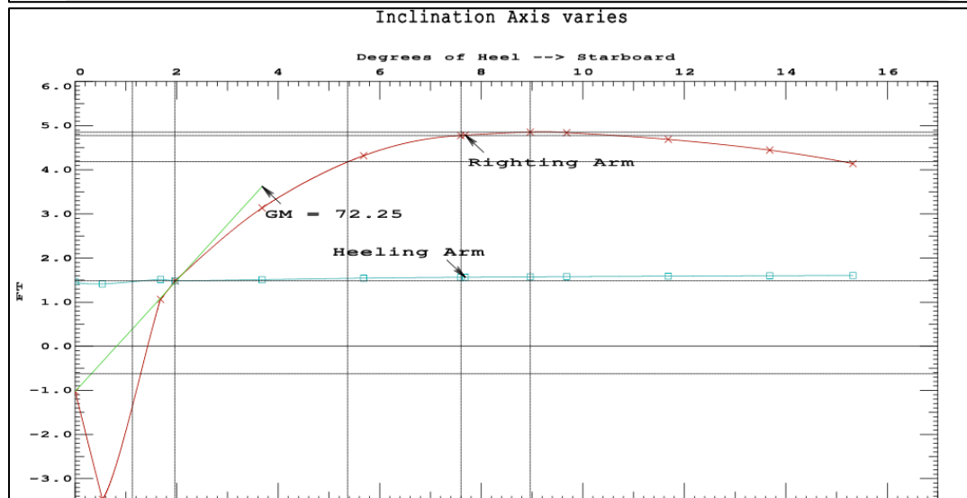
Figure 33: GHS output for varied axis analysis of casualty condition with 60-knot winds. Note that axis angles in GHS are measured clockwise from 270° relative.
