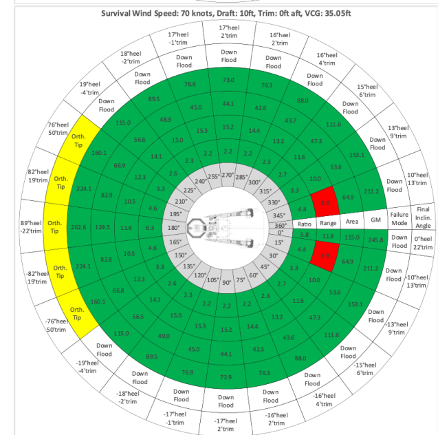
Figure 16: MSC Fixed Interval Analysis Results for 60-knot wind (left) and 70-knot wind (right). 9.5-foot draft (top), 10-foot draft (bottom). Trim is zero
